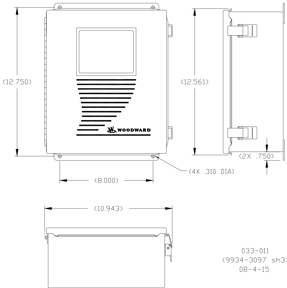
GECO Vista Outline Drawing (Do not use for construction)
